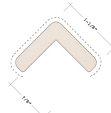
1010-OUTSIDE CORNER Core: POPLAR Wrapped Surface
