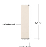
1016-LIGHT VALANCE Core: MDF Wrapped Surface
